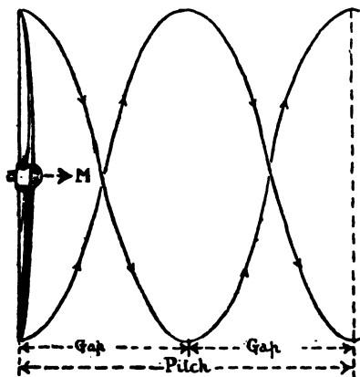
SPIRAL COURSES OF TWO-BLADE TIPS.
